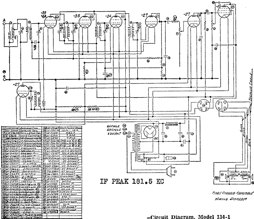
-Circuit Diagram, Model 134-1
